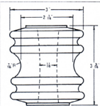
WK-913 Spool Insulator NEMA 53-3
