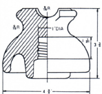
WK-1031 EEI-NEMA 55-3 Pin Type Insulator
