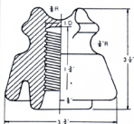
WK-1030 EEI-NEMA 55-2 Pin Type Insulator
