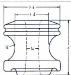
WK-912 Spool Insulator NEMA 53-2
