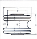
WK-914 Spool Insulator NEMA 53-4
