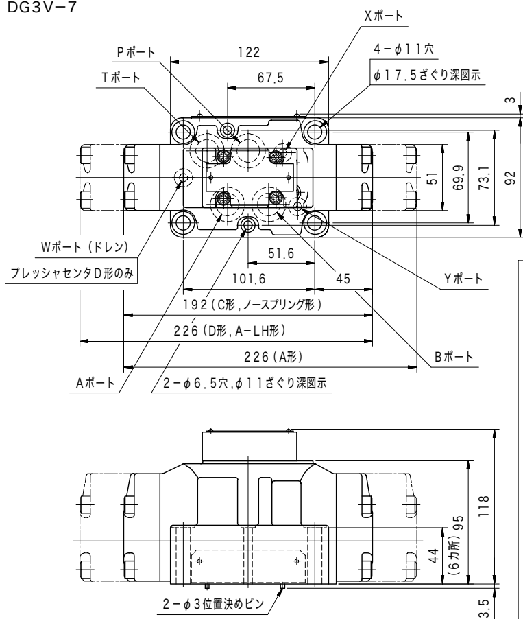
DG3V-7
