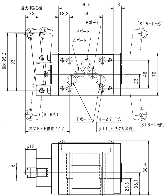
DG2S*-01*A-S15/S16
