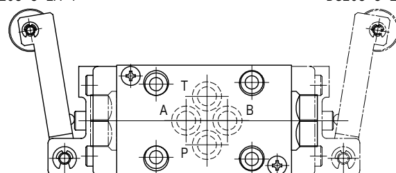
DG20S-3-2A-T
