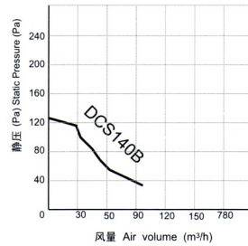
PERFORMANCE CURVES FOR "DCS" SERIES ("DCS"系列风量图)
